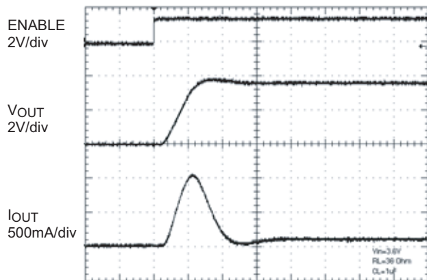
Turn-On Timing
