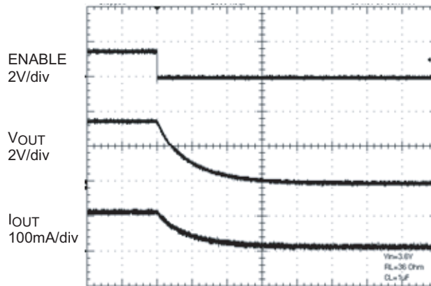
Turn-Off Timing
