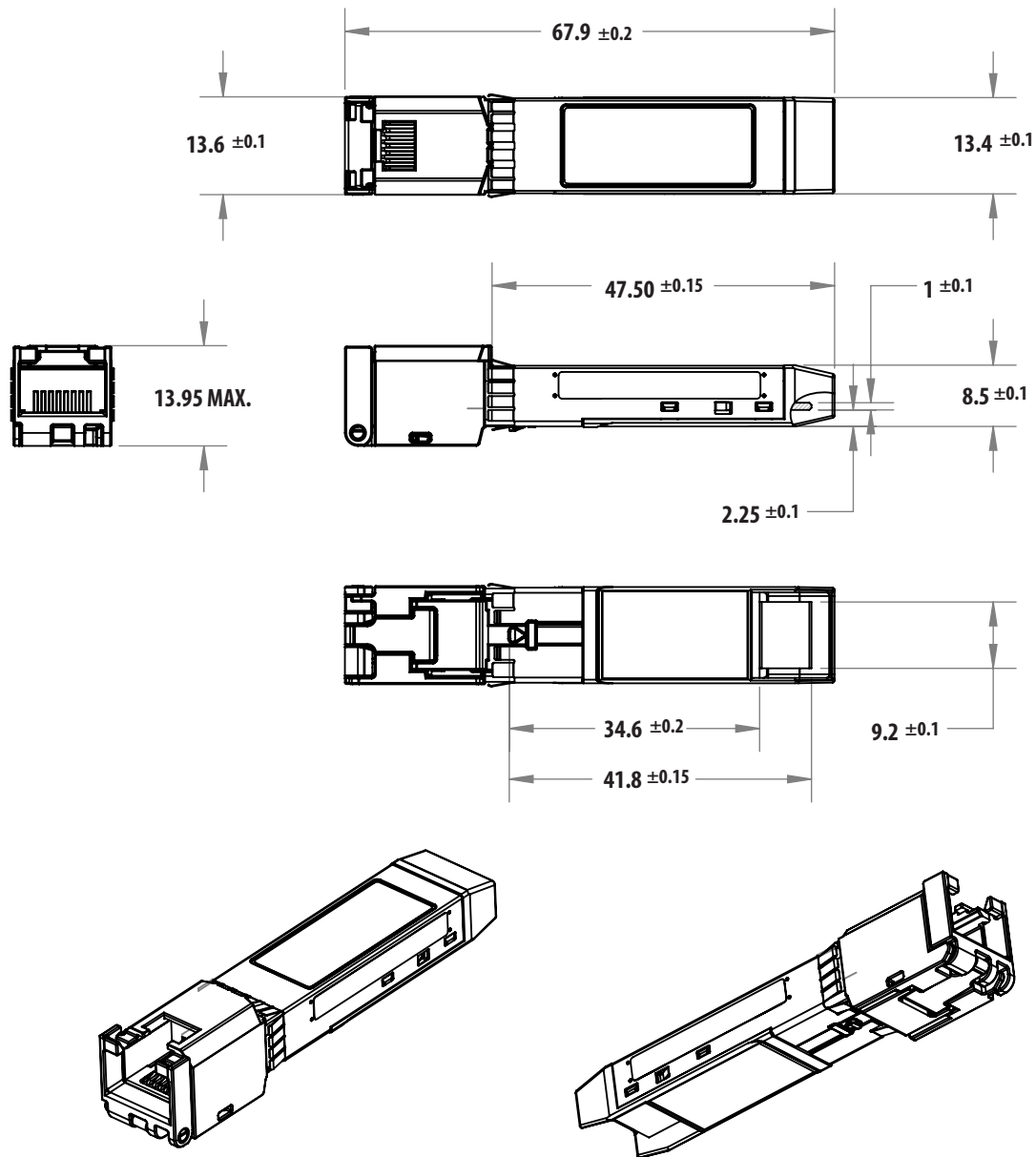
Figure 7. Module Drawing
