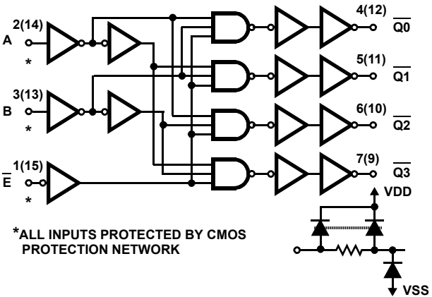
FIGURE 2. CD4556BMS LOGIC DIAGRAM (1 OF 2 IDENTICAL CIRCUITS)
