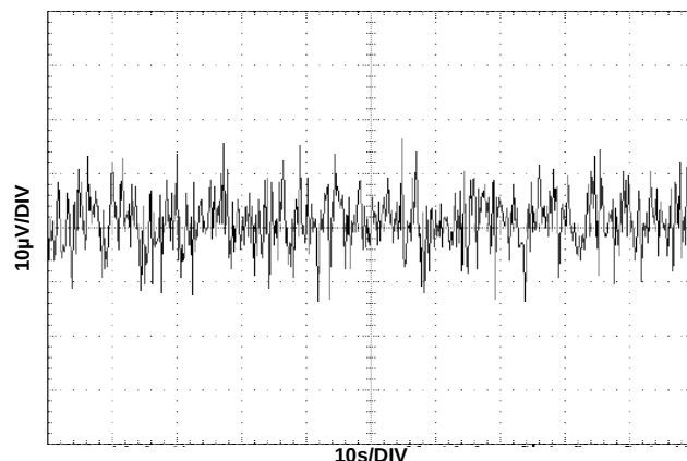
FIGURE 14. V_{OUT} NOISE
