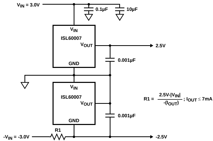
FIGURE 20. \pm 2.5V DUAL OUTPUT, HIGH ACCURACY REFERENCE
