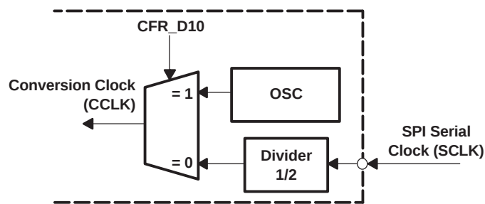
Figure 54. Converter Clock
