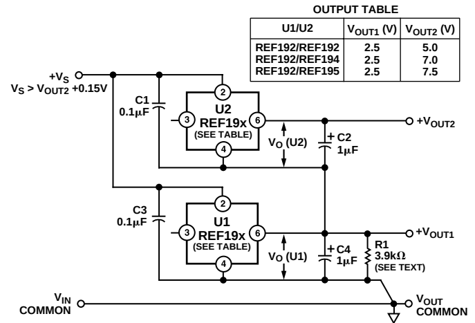
Figure 19. Stacking Voltage References with the REF19x
