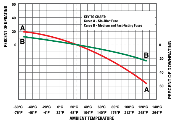
Figure 2 – Fuse Rerating Curve
