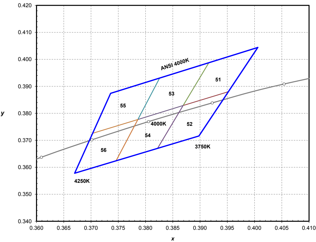
Figure 18. ANSI 4000K 1/6th color bin structure.
