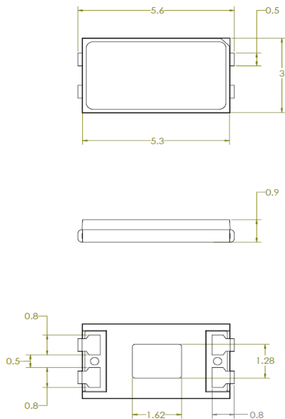
Figure 1. Package outline drawing.
