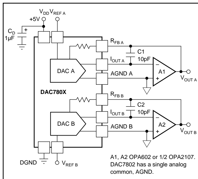
FIGURE 3. Unipolar Configuration.
