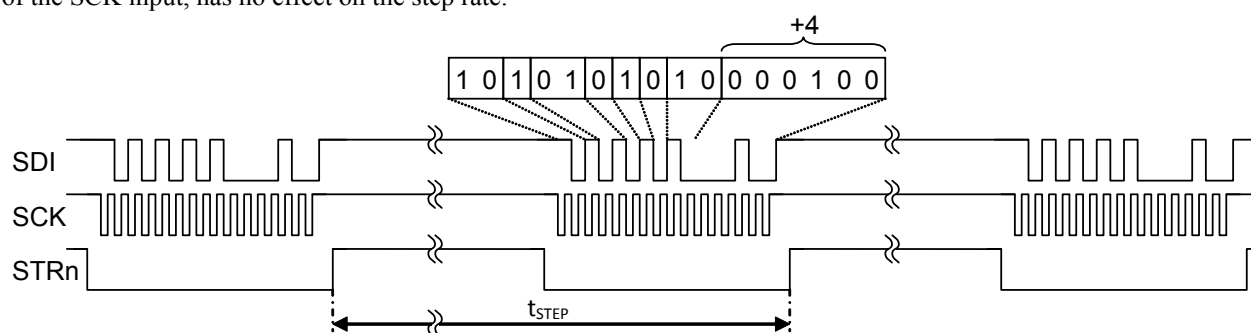
Figure 11: Serial Interface Sequence for Quarter Step in Forward Direction
