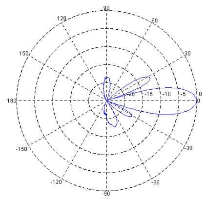
H-field radiation pattern (azimuth for vertically polarized antenna)
