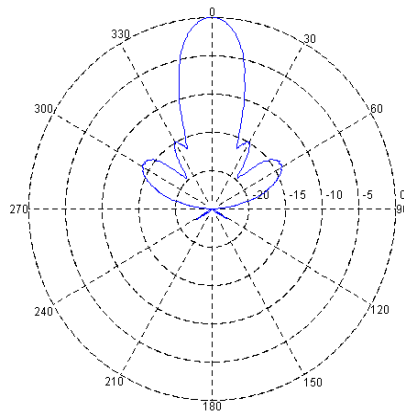
E-field radiation pattern (azimuth for horizontally polarized antenna)
