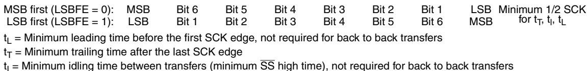
Figure 14-10. SPI Clock Format 1 (CPHA = 1)
