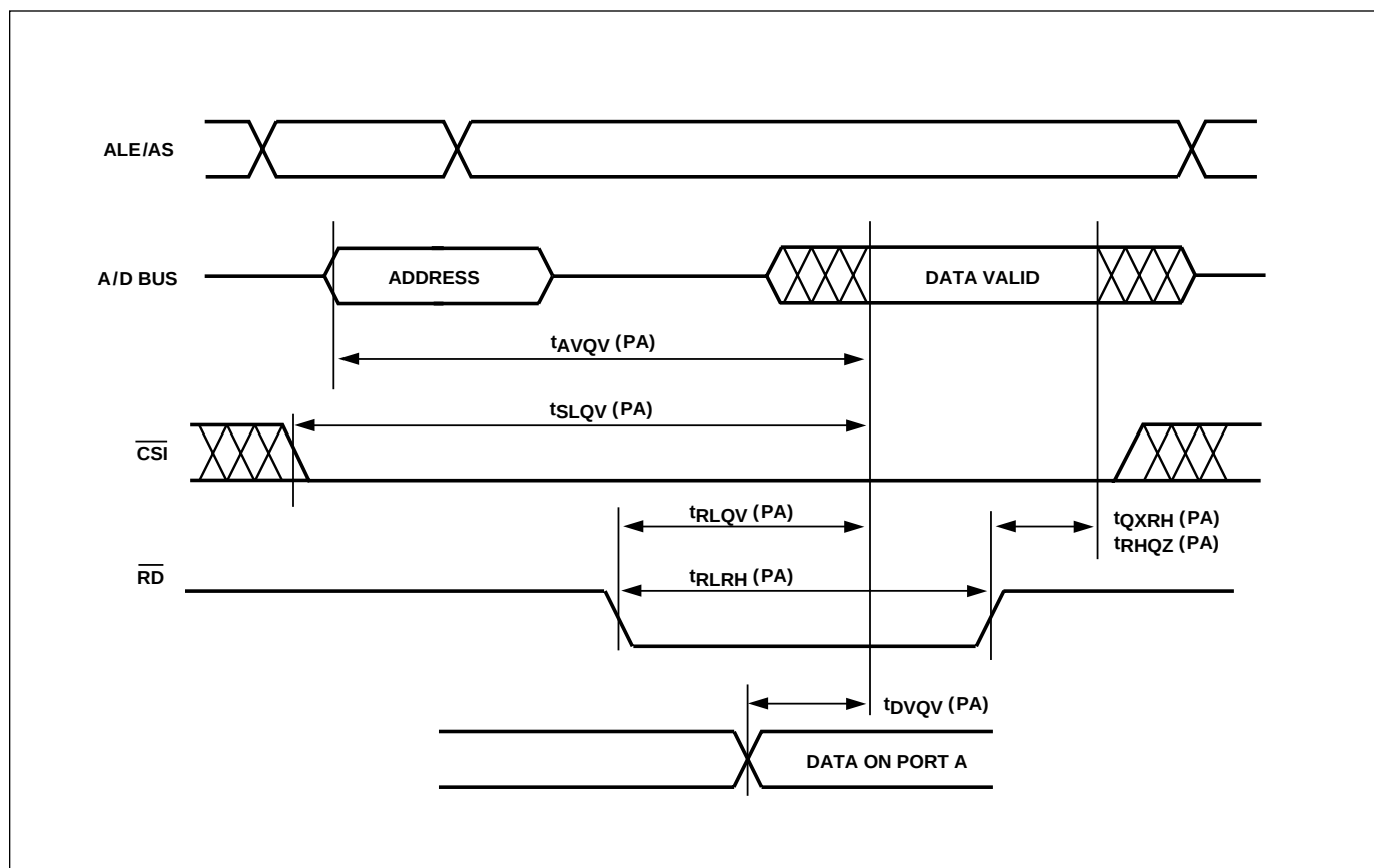
Figure 34. Peripheral I/O Read Timing
