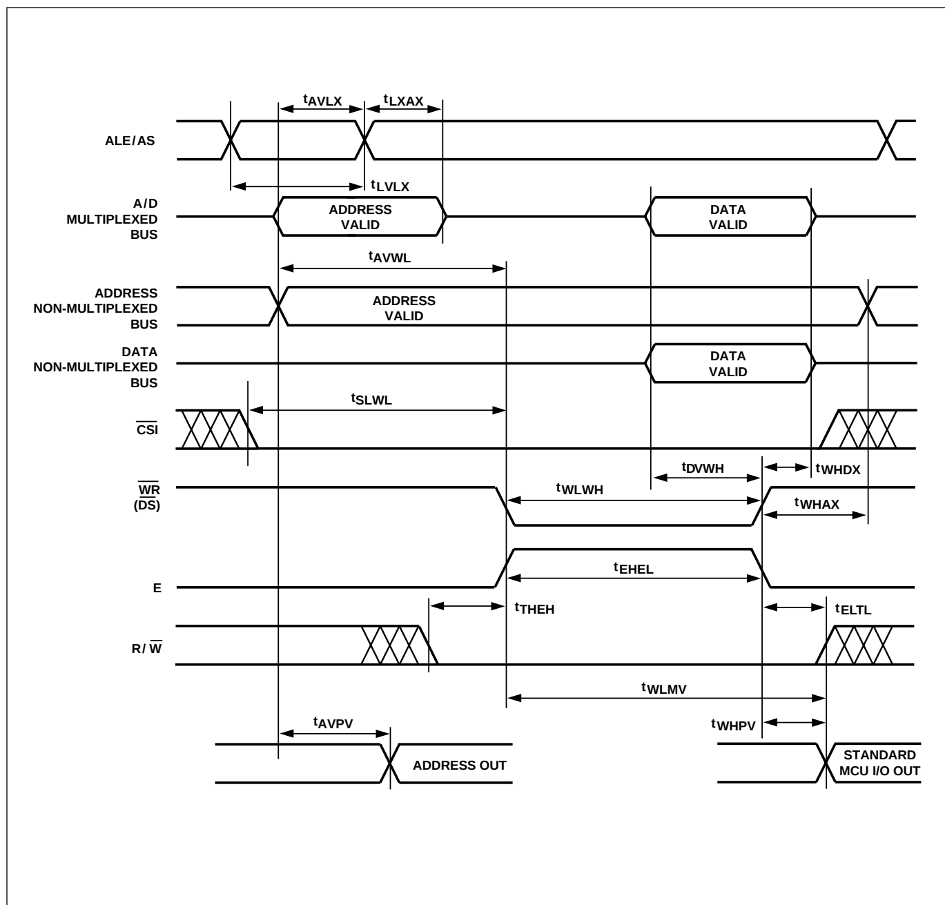
Figure 33. Write Timing
