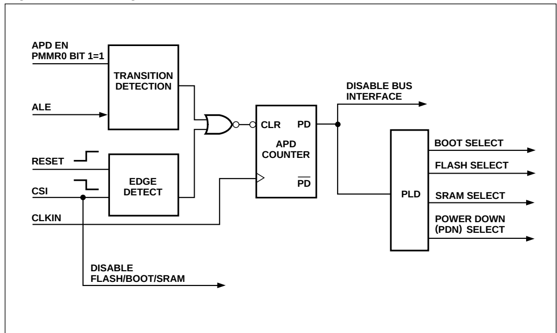
Figure 28. APD Logic Block
