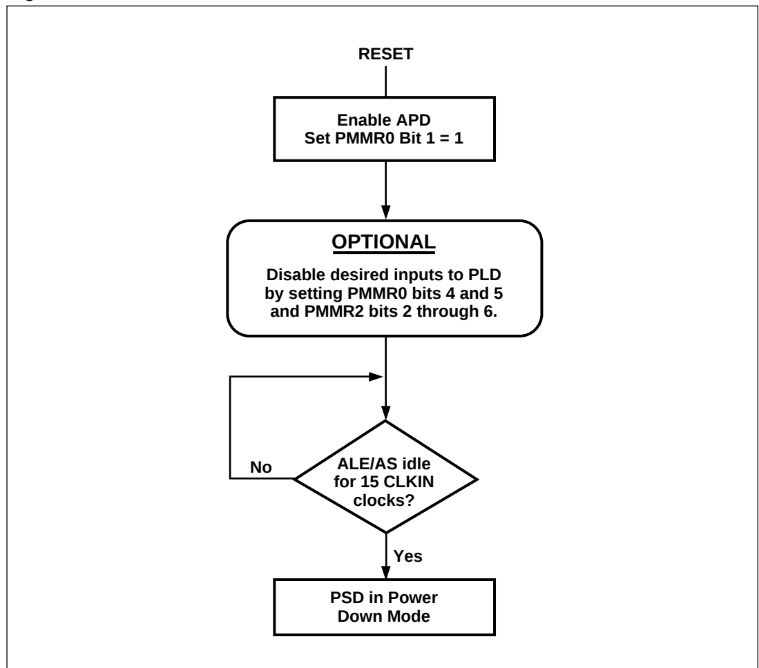
Figure 29. Enable Power Down Flow Chart
