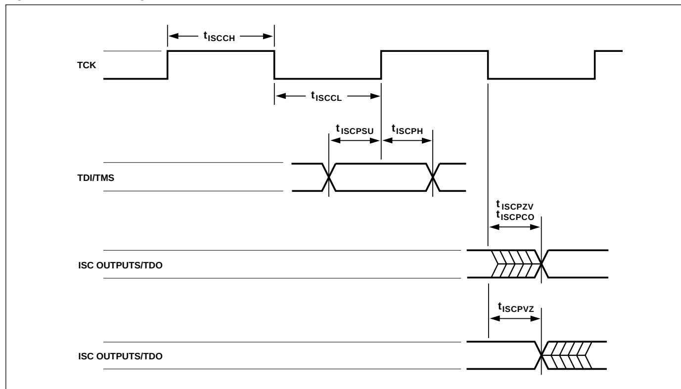
Figure 42. ISC Timing
