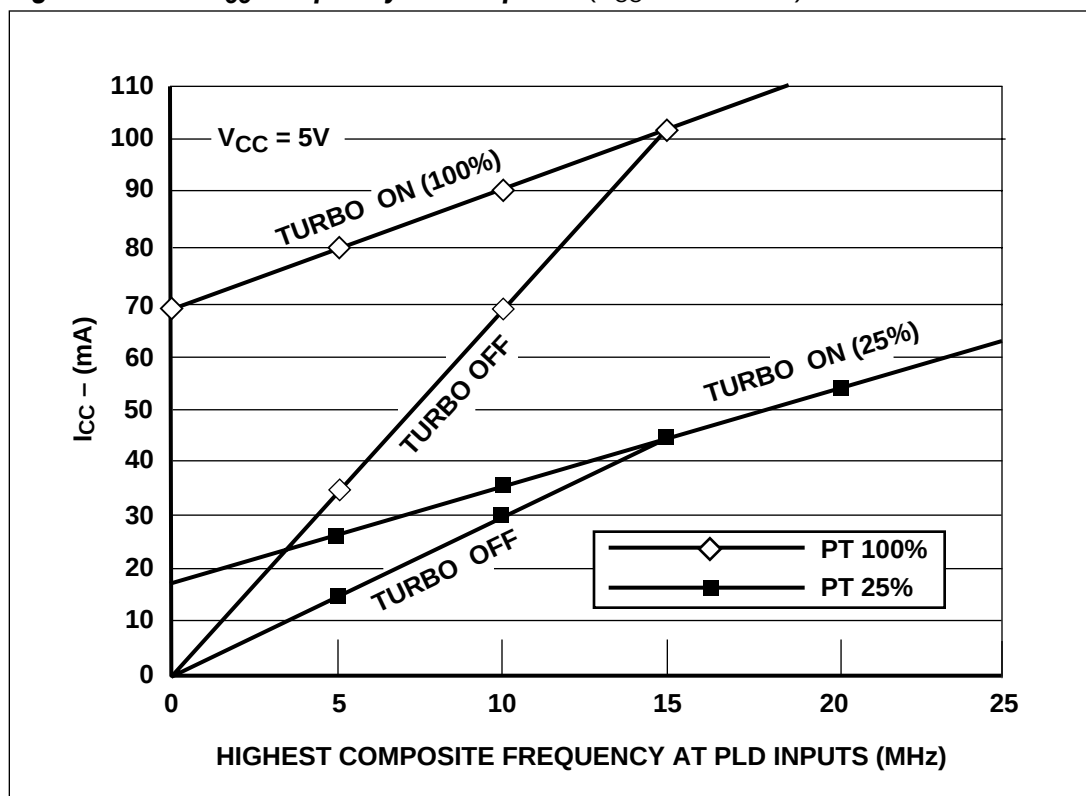
Figure 31. PLD I_{CC} /FrequencyConsumption ( V_{CC} = 5\text{ V} \pm 10\% )
