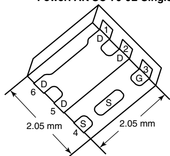
PowerPAK SC-70-6L-Single
