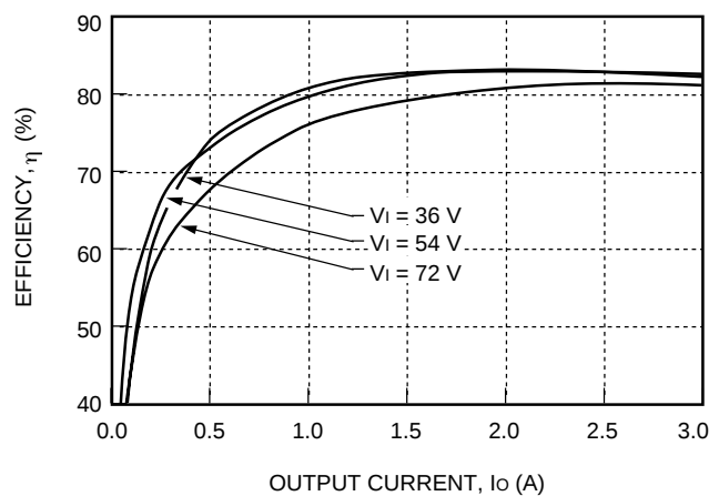
Figure 14. CW030B-M Typical Converter Efficiency vs. Output Current
