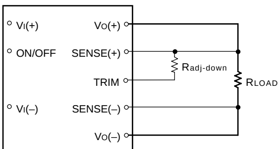
Figure 25. Circuit Configuration to Decrease Output Voltage
