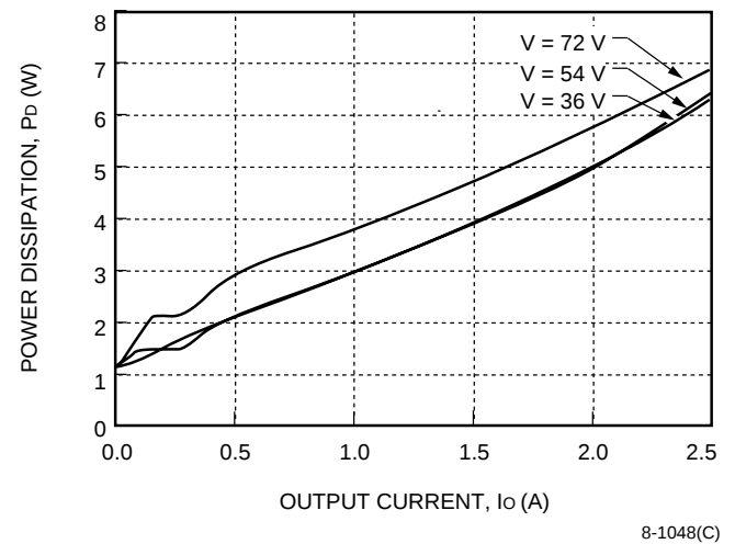
Figure 30. CW030B Power Dissipation vs. Output Current
