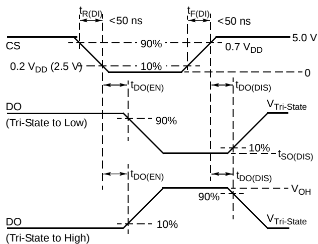
Figure 11. Turn-ON/OFF Waveforms
