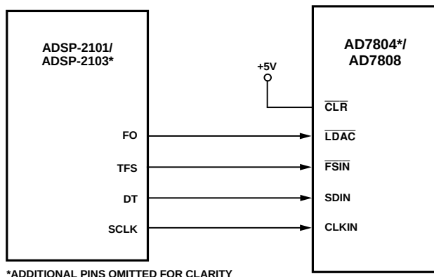
Figure 35. ADSP-2101/ADSP-2103 Interface
