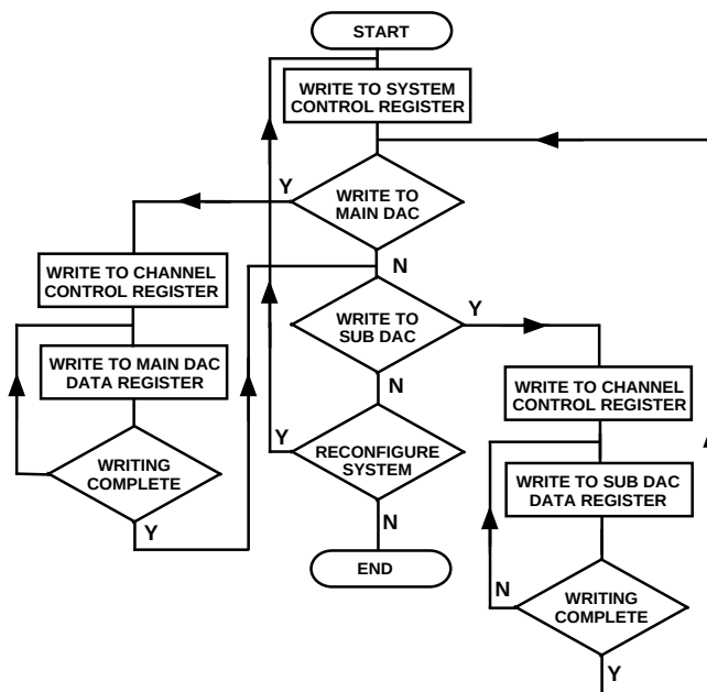
Figure 19. Flowchart for Controlling the AD7805/AD7809 DACs in 10-Bit Parallel Mode Following Power-Up
