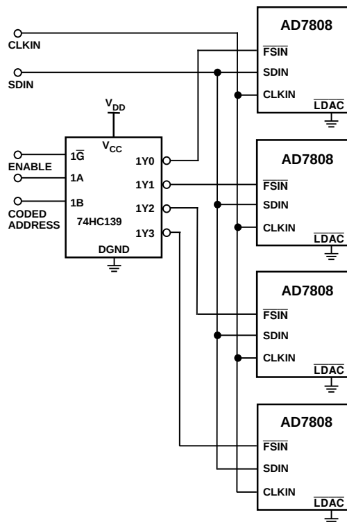
Figure 42. Decoding Multiple AD7808s Using the FSIN Pin
