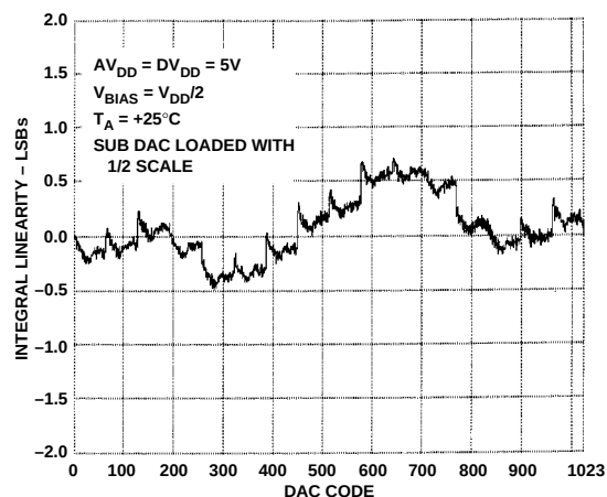
Figure 32. Integral Linearity with 5 V Operation
