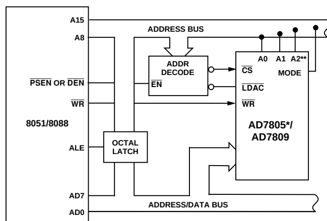
Figure 40. AD7805/AD7809–8051/8088 Interface
