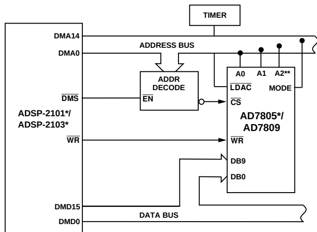
Figure 38. AD7805/AD7809–ADSP-2101/ADSP-2103 Interface
