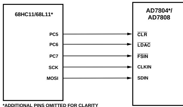
Figure 36. AD7804/AD7808–68HC11/68L11 Interface
