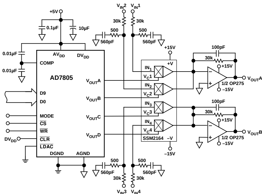
Figure 44. Low Cost, Two-Channel Mixer
