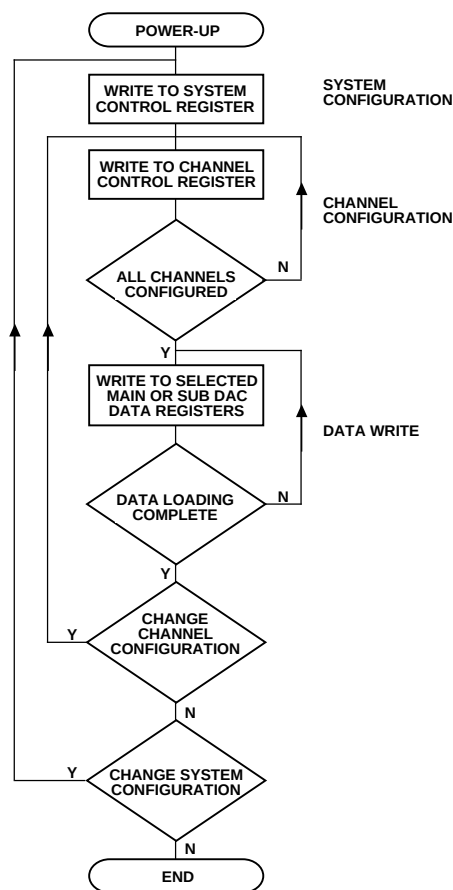
Figure 10. Flowchart for Controlling the DAC Following Power-Up
