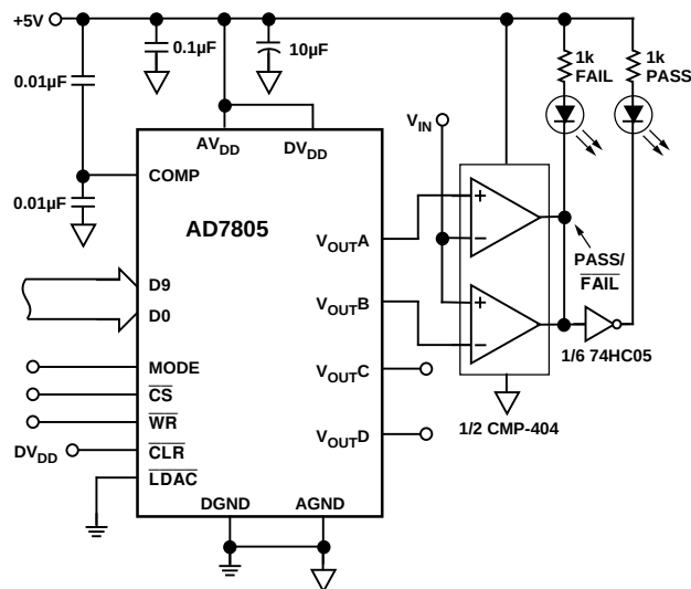
Figure 43. Digitally Programmable Window Detector
