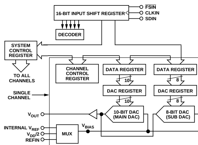
Figure 3. AD7804/AD7808 Internal Registers
