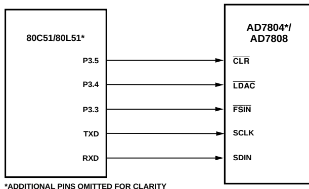
Figure 37. AD7804/AD7808–80C51/80L51 Interface
