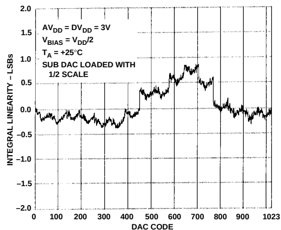
Figure 33. Integral Linearity with 3 V Operation
