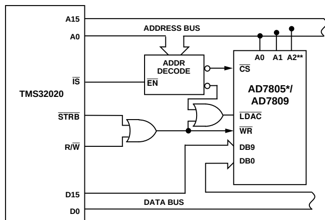
Figure 39. AD7805/AD7809–TMS32020 Interface
