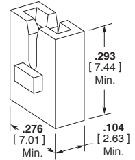
Cavity Specification 1601434
