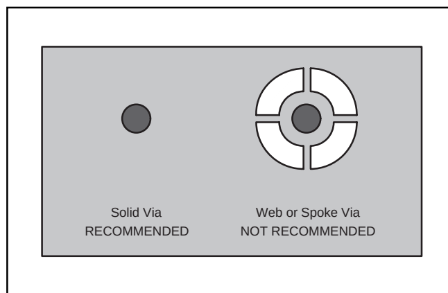
FIGURE 17. Via Connection.
