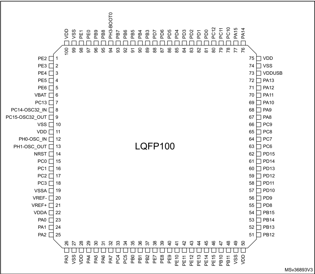
Figure 6. STM32L433Vx LQFP100 pinout (1)
