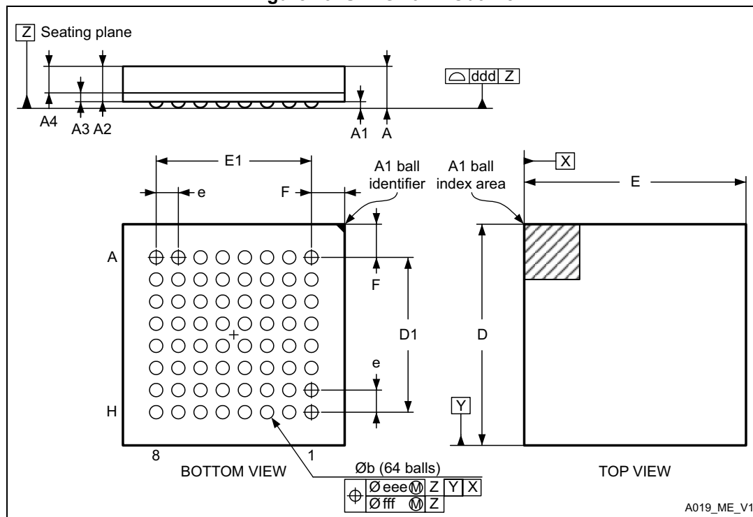
Figure 49. UFBGA64 – Outline
