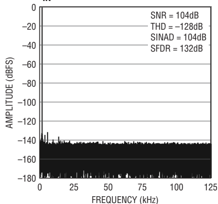
128k Point FFT f_S = 250\text{kps} , f_{IN} = 2\text{kHz}
