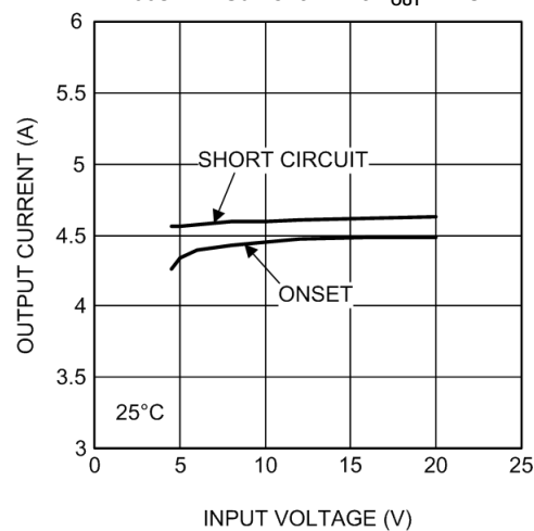
LMZ12003EXT Current Limit V_{OUT} = 1.8\text{V}
