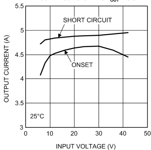
LMZ14203EXT Current Limit V_{OUT} = 3.3\text{V}
