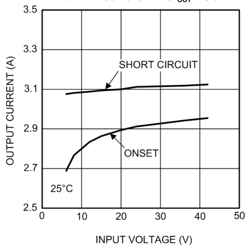
LMZ14202EXT Current Limit V_{OUT} = 3.3\text{V}
