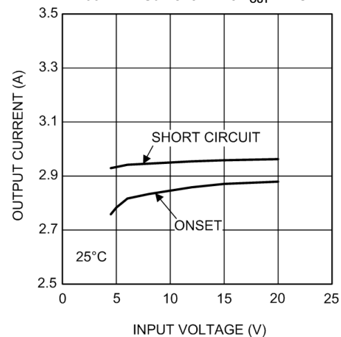
LMZ12002EXT Current Limit V_{OUT} = 1.8\text{V}
