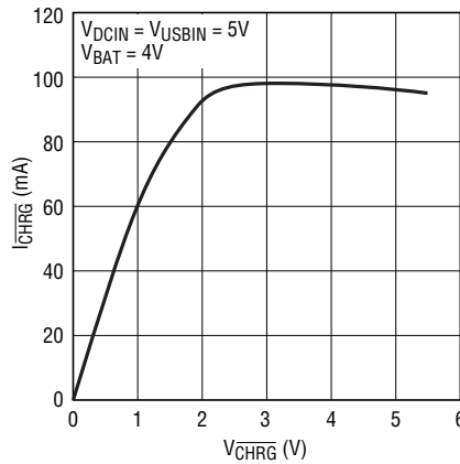
CHRG Pin I-V Curve
