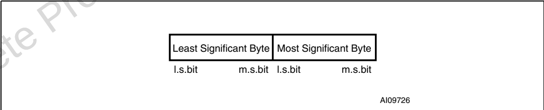
Figure 15. CRC format
