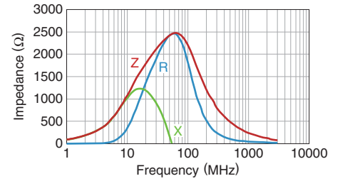
MMZ1608Y600B
