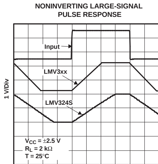
1 μs/Div Figure 27.
