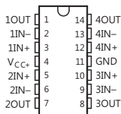
LMV324 . . . D (SOIC) OR PW (TSSOP) PACKAGE (TOP VIEW)
