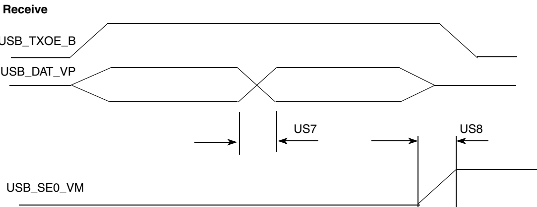
Figure 101. USB Receive Waveform in DAT_SE0 Bidirectional Mode
