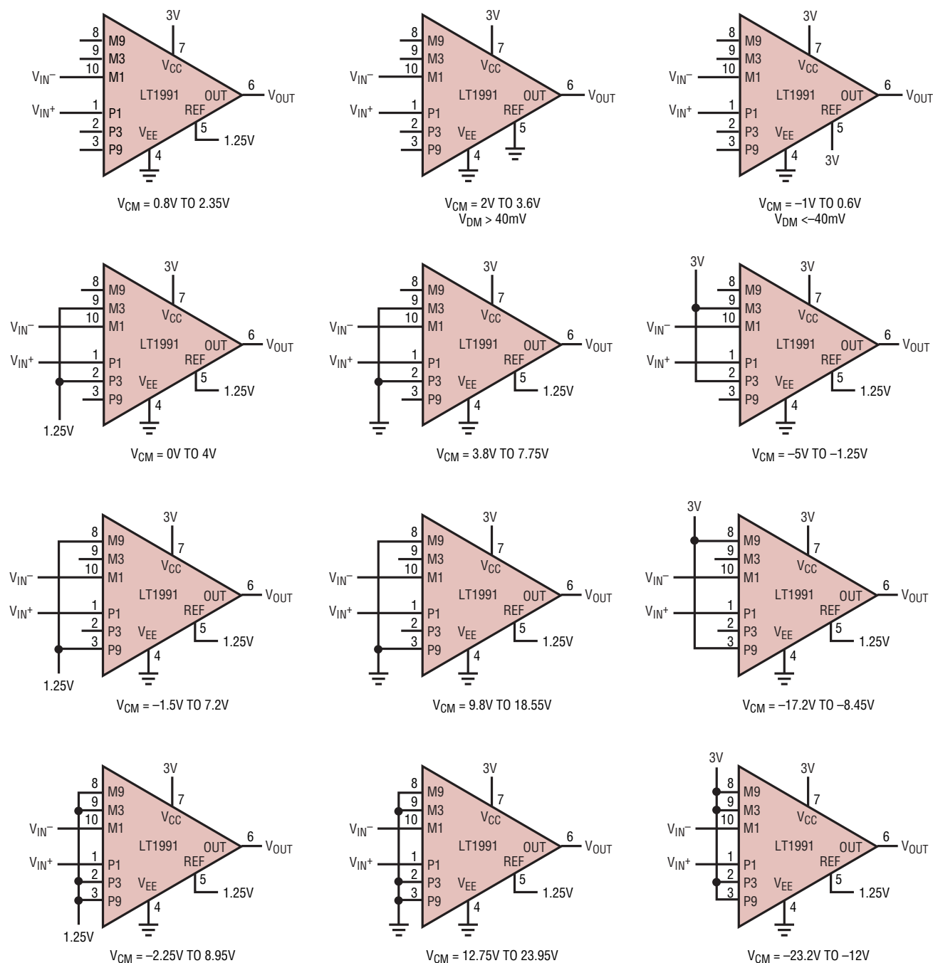
Figure 15. Common Mode Ranges for Various LT1991 Configurations on V_S = 3\text{V} , 0\text{V} ; with Gain = 1
