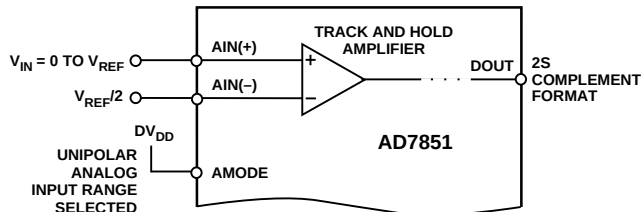
Figure 15. \pm V_{REF}/2 about V_{REF}/2 Bipolar Input Configuration
