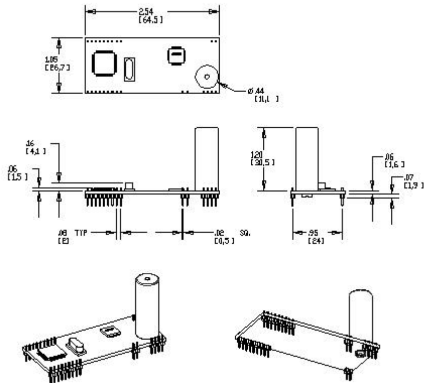
Figure 2 - CC-900W Integrated antenna model (-A)
