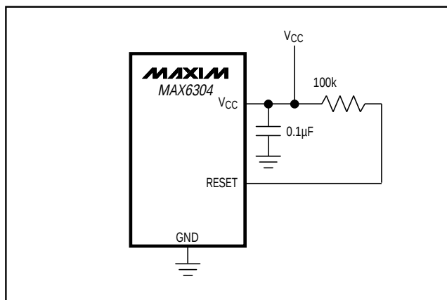
Figure 10. Ensuring RESET Valid to V_{CC} = 0V
