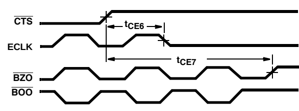
FIGURE 13. ENCODER TIMING
