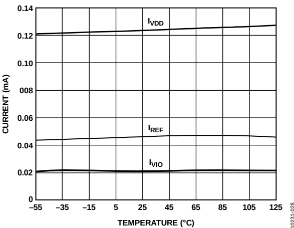
Figure 27. Operating Currents vs. Temperature (AD7988-1)
