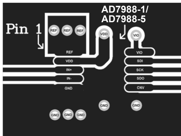
Figure 42. Example Layout of the AD7988-1/AD7988-5 (Top Layer)
