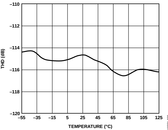
Figure 25. THD vs. Temperature
