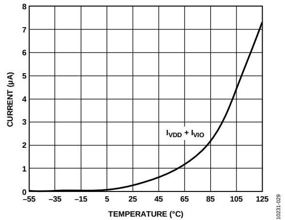
Figure 28. Power-Down Currents vs. Temperature
