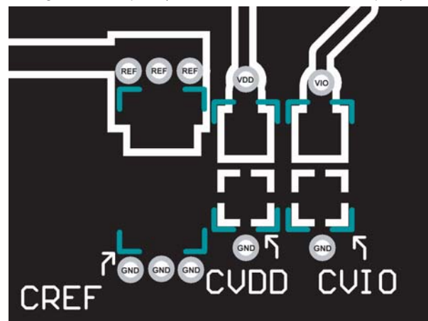
Figure 43. Example Layout of the AD7988-1/AD7988-5 (Bottom Layer)
