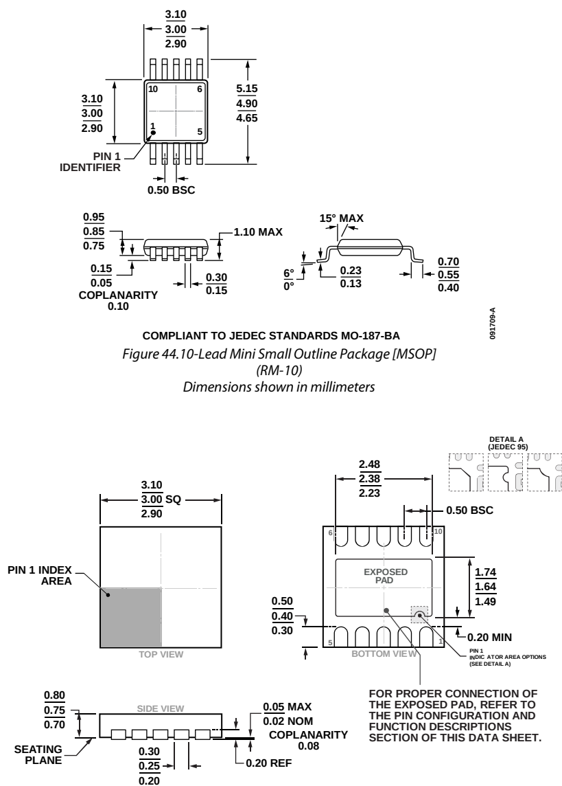
Figure 45. 10-Lead Lead Frame Chip Scale Package [LFCSP] 3 mm × 3 mm Body and 0.75 mm Package Height (CP-10-9)
