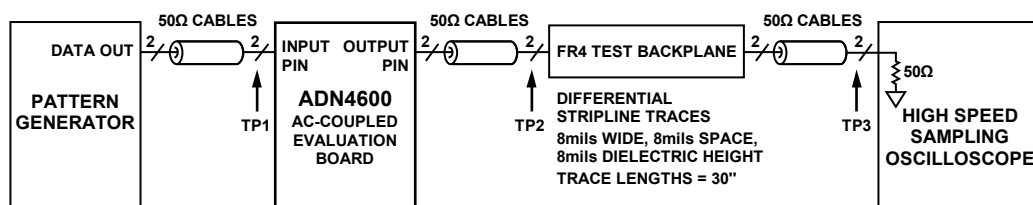
Figure 14. Output Pre-Emphasis Test Circuit, FR4
