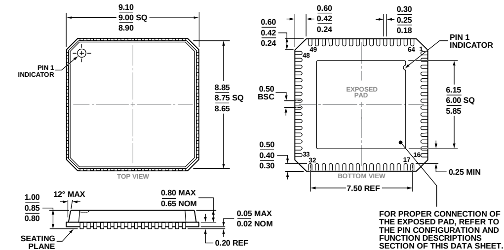
Figure 33. 64-Lead Lead Frame Chip Scale Package [LFCSP_VQ] 9 mm × 9 mm Body, Very Thin Quad (CP-64-2) Dimensions shown in millimeters
