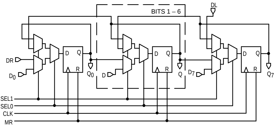
LOGIC DIAGRAM
