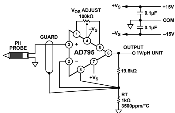
Figure 50. pH Probe Amplifier
