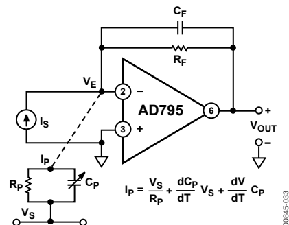
Figure 33. Sources of Parasitic Leakage Currents
