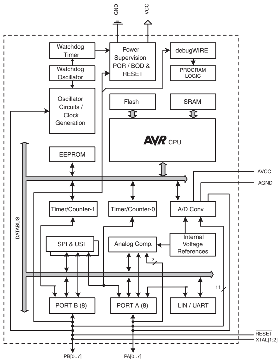
Figure 1-1. Block Diagram
