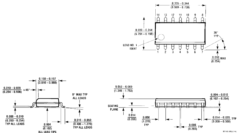
14-Lead Small Outline Molded Package (M) Order Number DM74LS27M Package Number M14A
