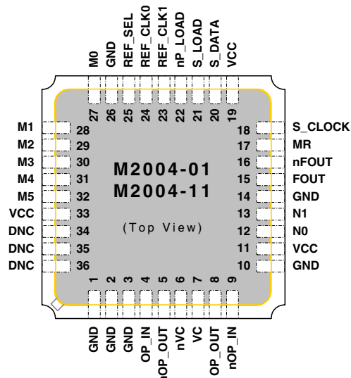
Figure 1: Pin Assignment
