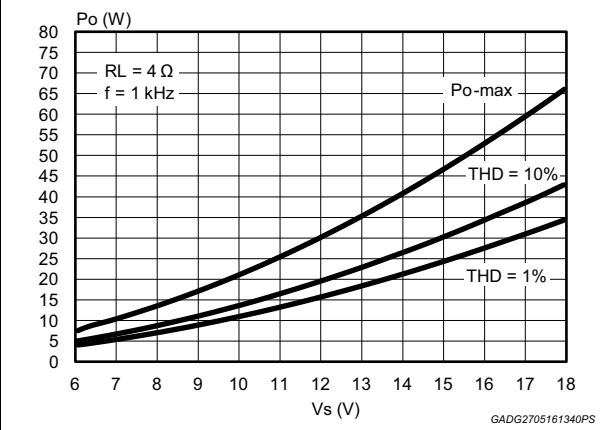
Figure 6. Output power vs. supply voltage (4 \Omega )
