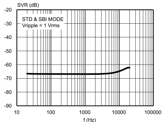
Figure 22. Supply voltage rejection vs. frequency
