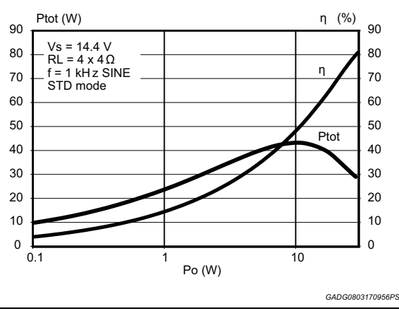
Figure 23. Total power dissipation & efficiency vs. Po (4 Ω, STD, Sine)
