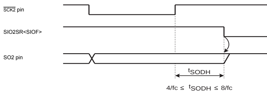
Figure 15-8 Hold Time of the End of Transmit Mode
