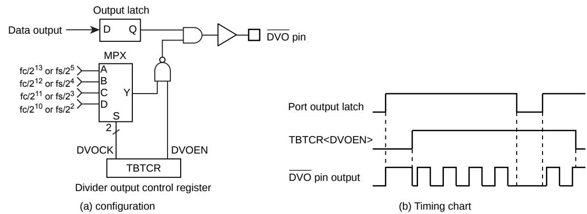
Figure 7-3 Divider Output
