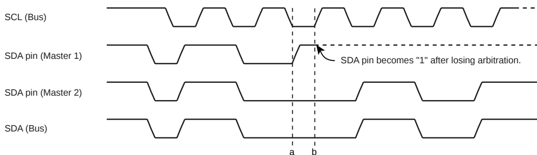
Figure 16-7 Arbitration Lost
