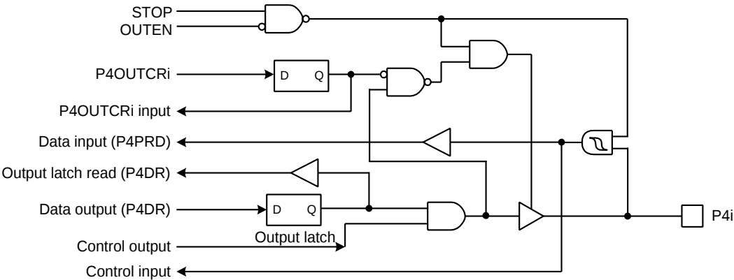
Figure 5-6 Port 4
