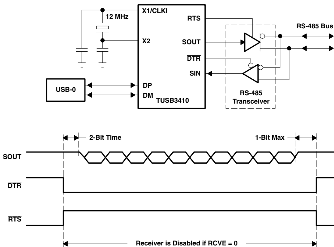
Figure 3-3. RS-485 Bus Implementation
