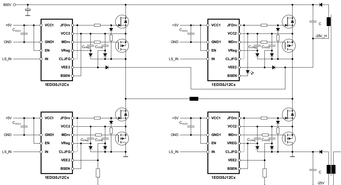
Figure 7 Application drawing for high side bootstrap supply (FB)
