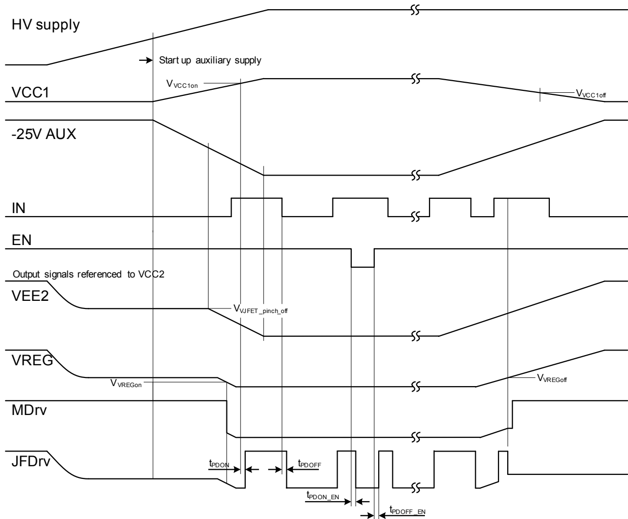
Figure 6 Principle start up with the auxiliary supplies not present when voltage is applied over the switch (Signal names are chosen equivalent to the pin names of the driver)
