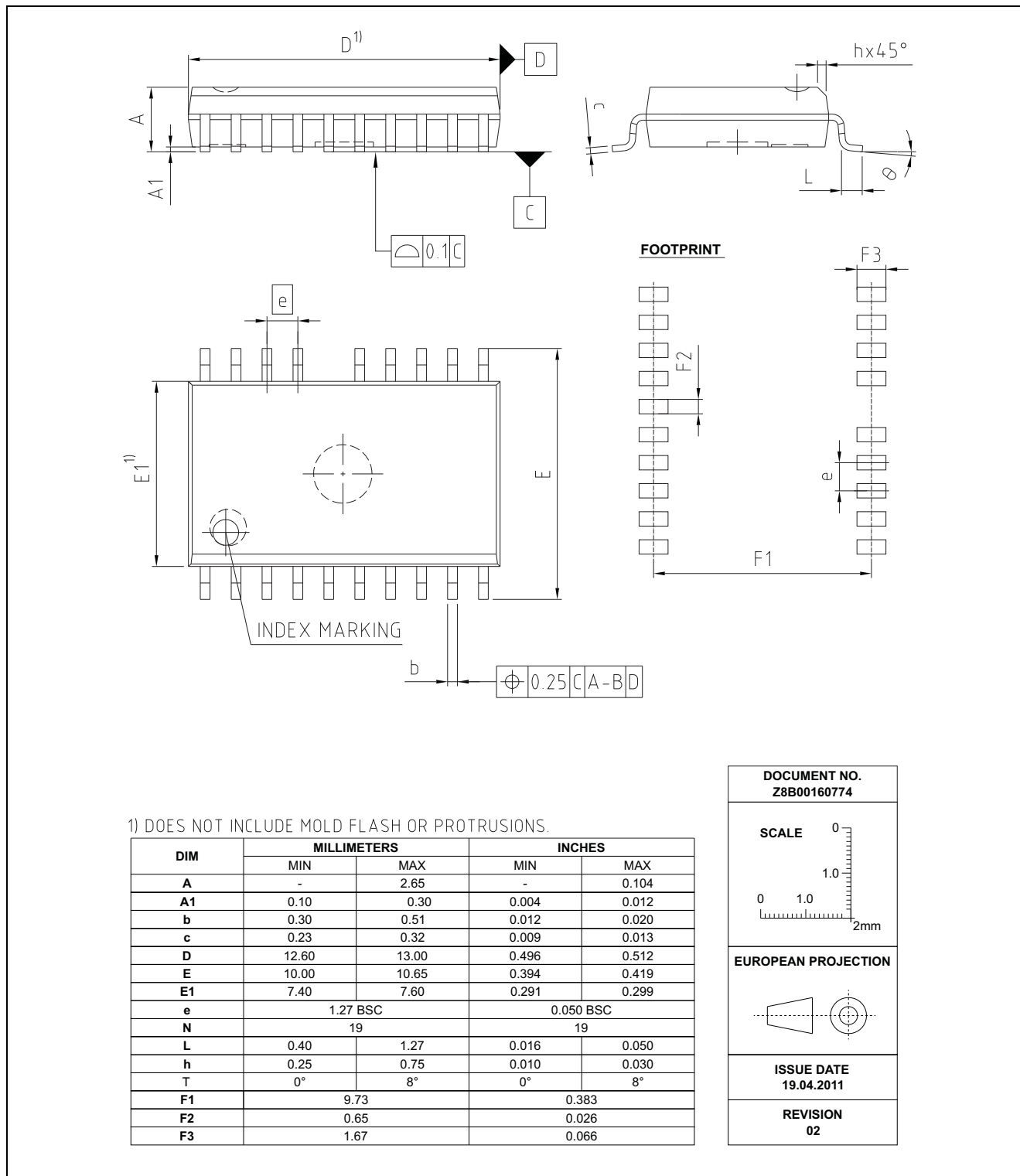
Figure 11 PG-DSO-19-4
