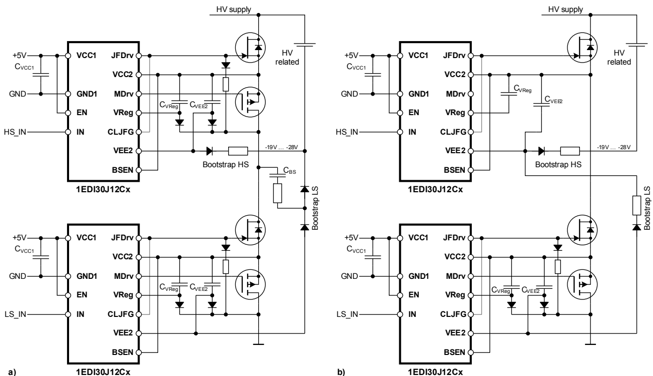
Figure 15 Cascaded bootstrap supply, a) cascode configuration, b) only JFET
