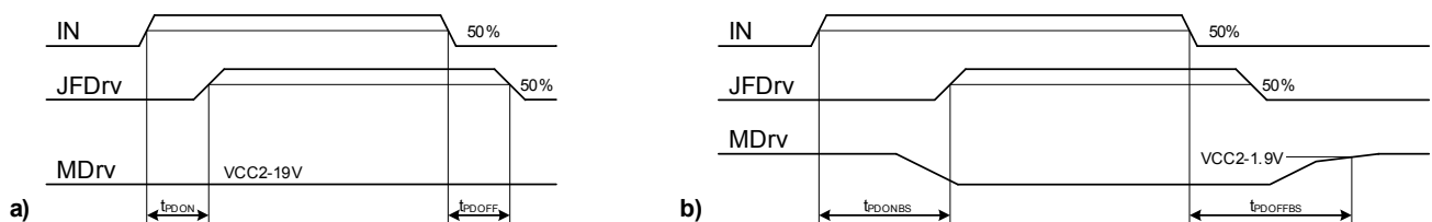
Figure 9 Timing of IN to JFDrv, a) normal mode, b) bootstrap mode
