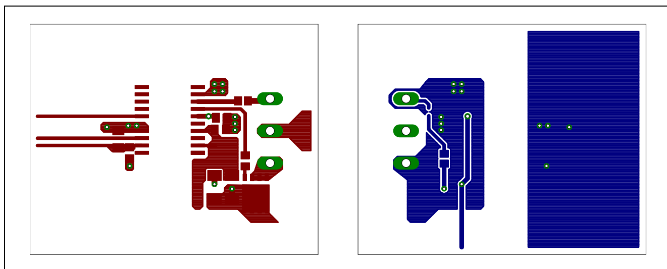
Figure 20 Thermal reference layout of a 1EDI30J12CP driver stage
