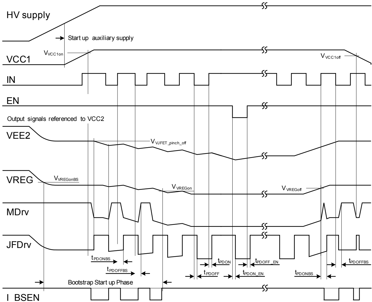
Figure 8 Start up bootstrap supply mode for high side located cascodes (BSEN connected to VCC2) (Signal names are chosen equivalent to the pin names of the driver)
