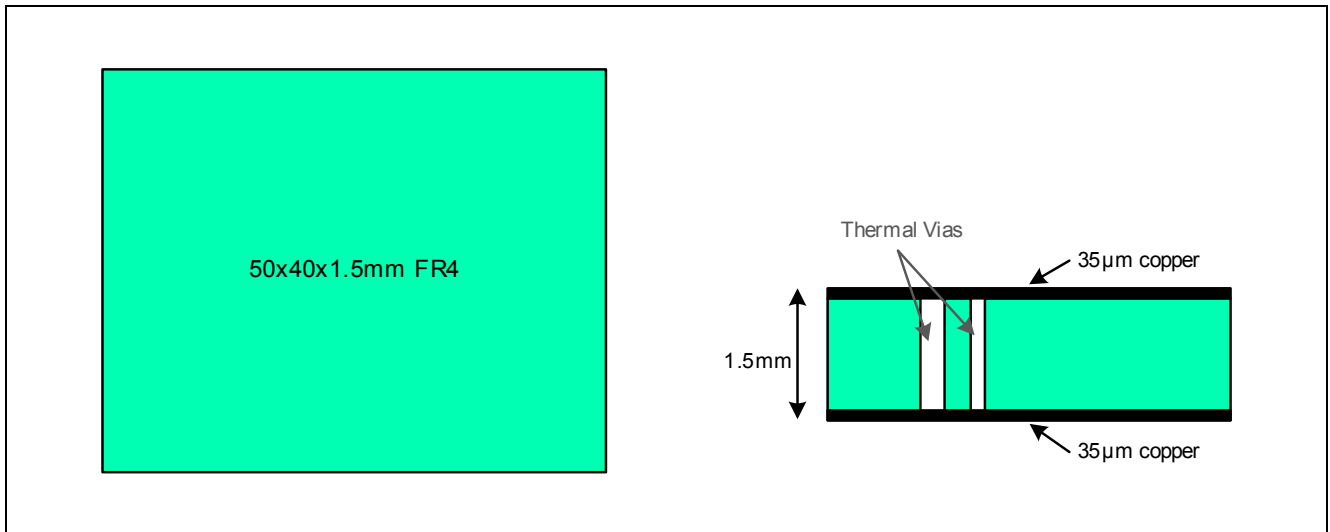
Figure 21 PCB Stack - Thermal reference layout
