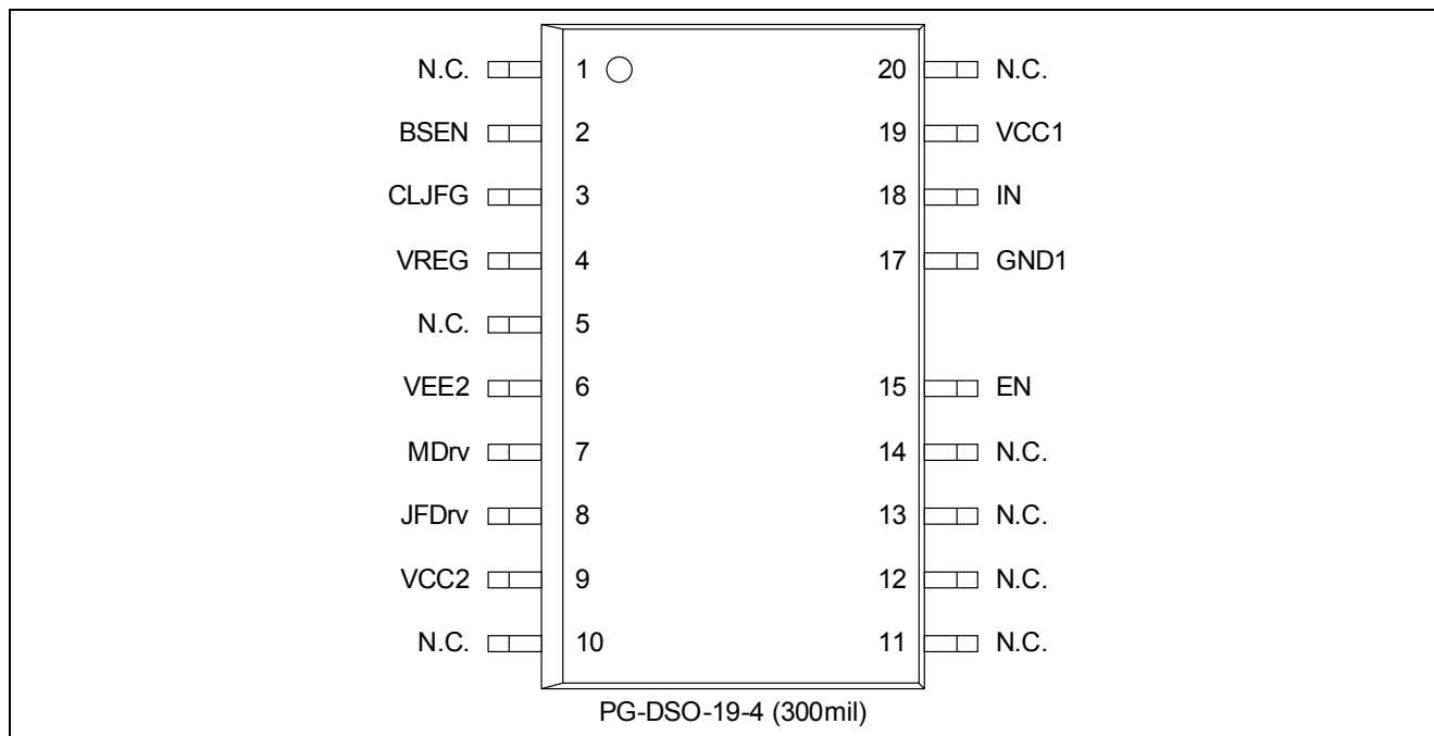
Figure 2 Pin Configuration PG-DSO-19-4
