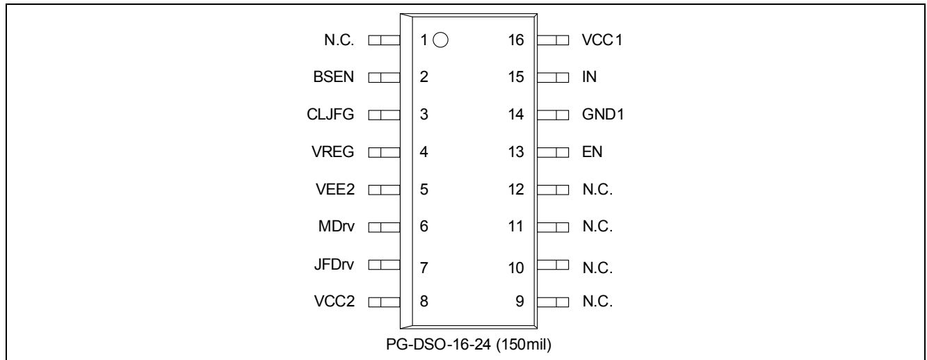
Figure 1 Pin Configuration PG-DSO-16-24
