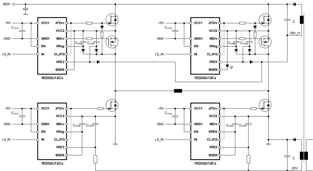
Figure 16 Application drawing for high side bootstrap supply (FB), low-side normally-on (refer to Figure 7 for low-side normally-off variant)
