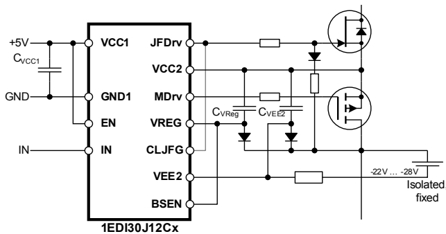
Figure 14 MOSFET drain related supply
