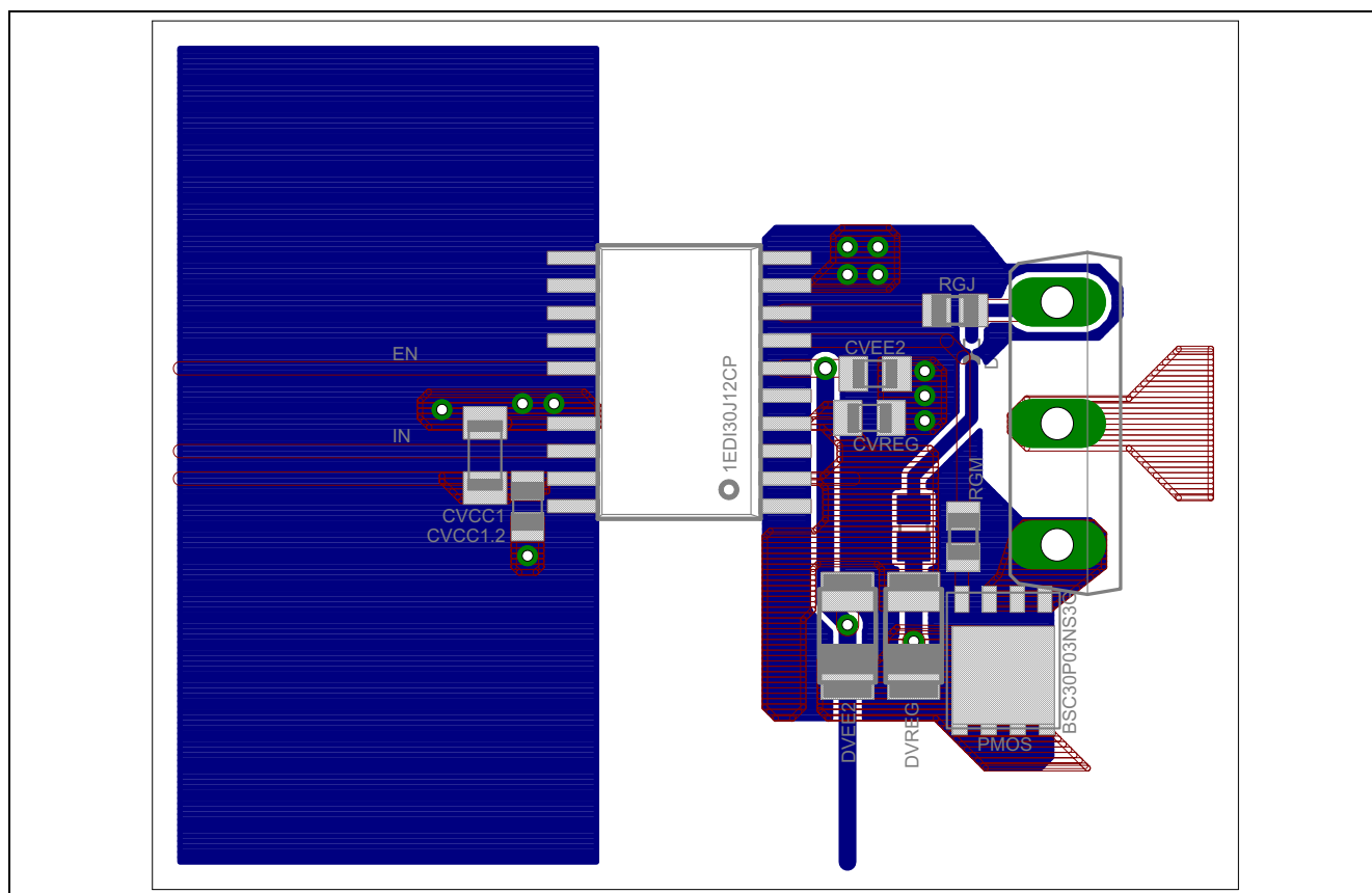
Figure 19 Typical layout of a 1EDI30J12CP driver stage
