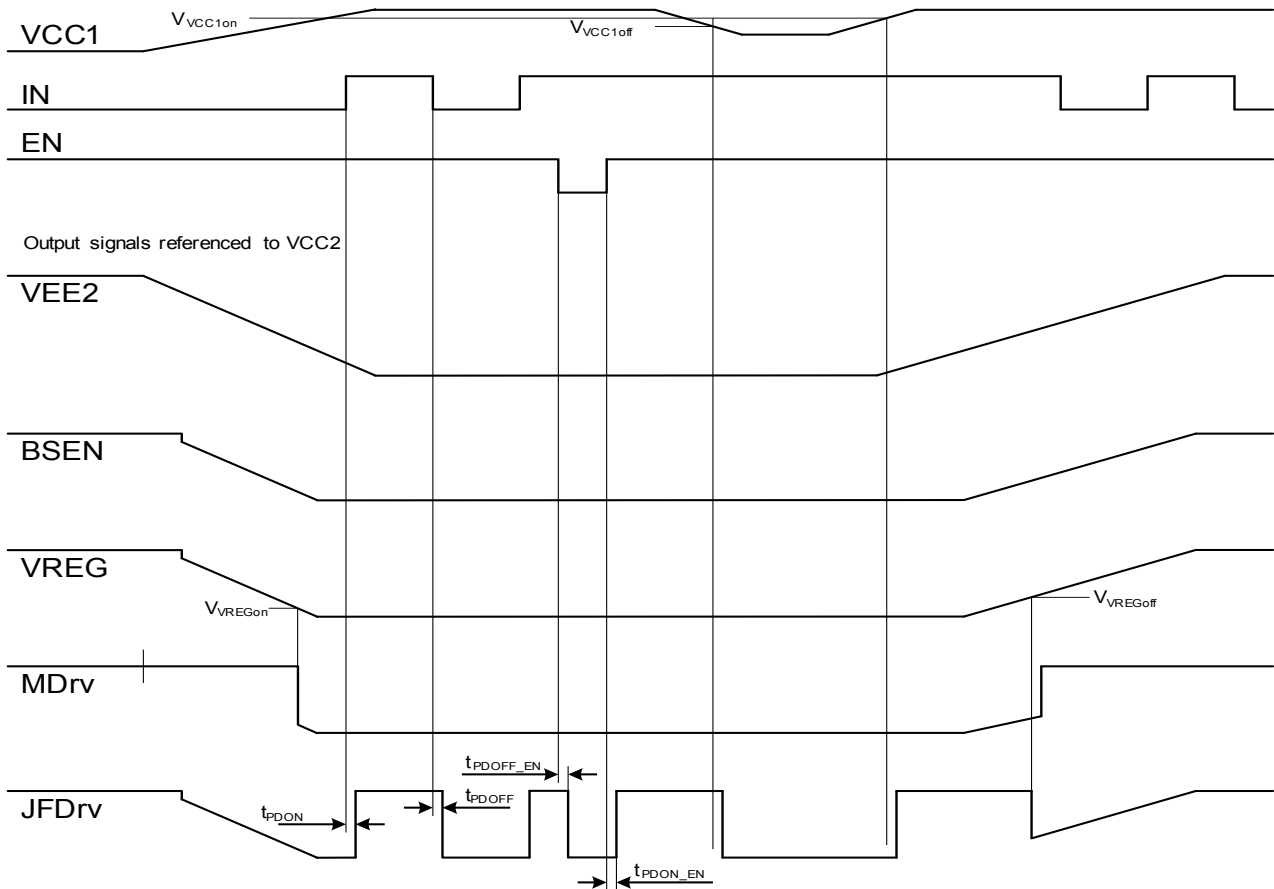
Figure 5 Principle start up, auxiliary supplies present before a voltage is applied over the switch (Signal names are chosen equivalent to the pin names of the driver)
