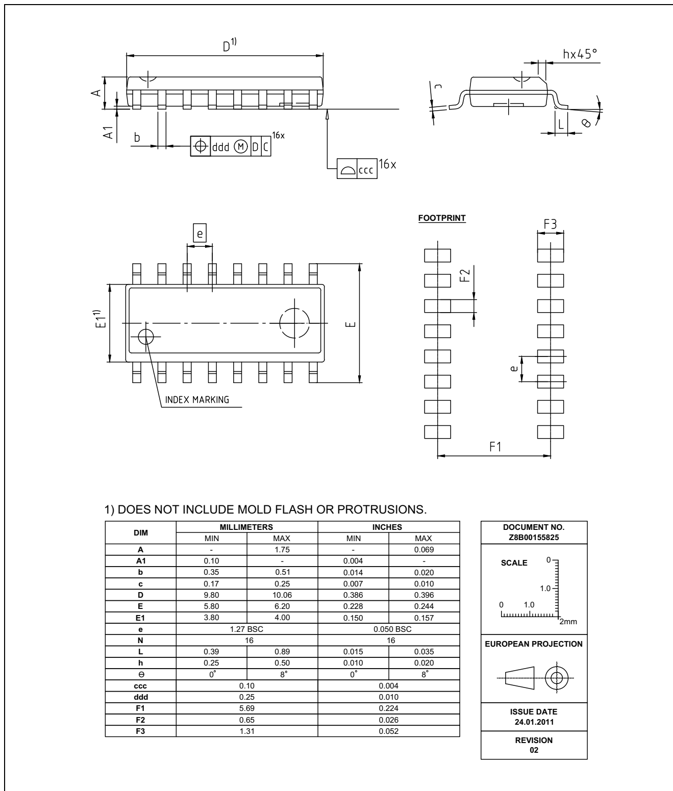
Figure 10 PG-DSO-16-24
