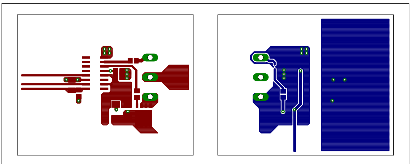
Figure 18 Thermal reference layout of a 1EDI30J12CL driver stage
