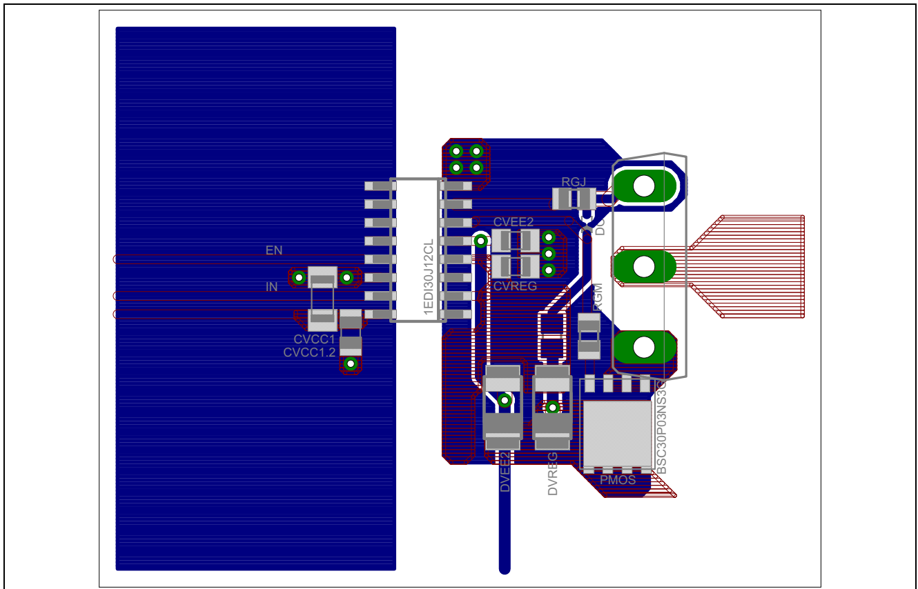
Figure 17 Typical layout of a 1EDI30J12CL driver stage
