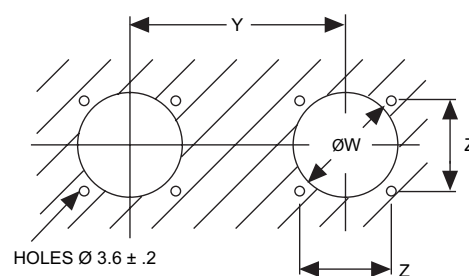
Panel Cutout
