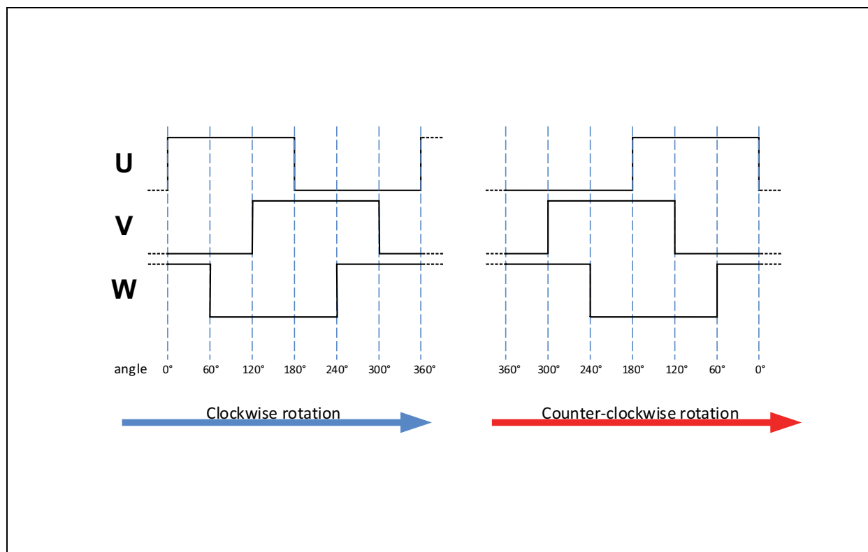
Figure 33: UVW Signals
