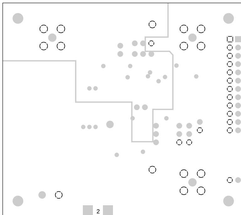
Fig 24. Printed-circuit board layout (ground layer)
