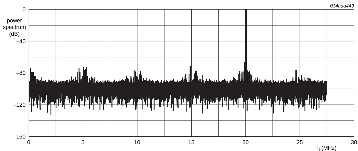
Fig 10. Two-tone; f_{i1} = 20 MHz; f_{i2} = 20.1 MHz; f_{clk} = 55 MHz
