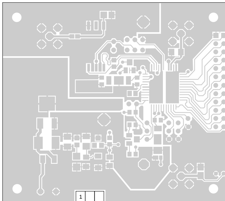
Fig 23. Printed-circuit board layout (top layer)
