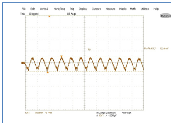
Figure 33: Output Voltage Ripple, 12A Load, Ch 1 :Vout
