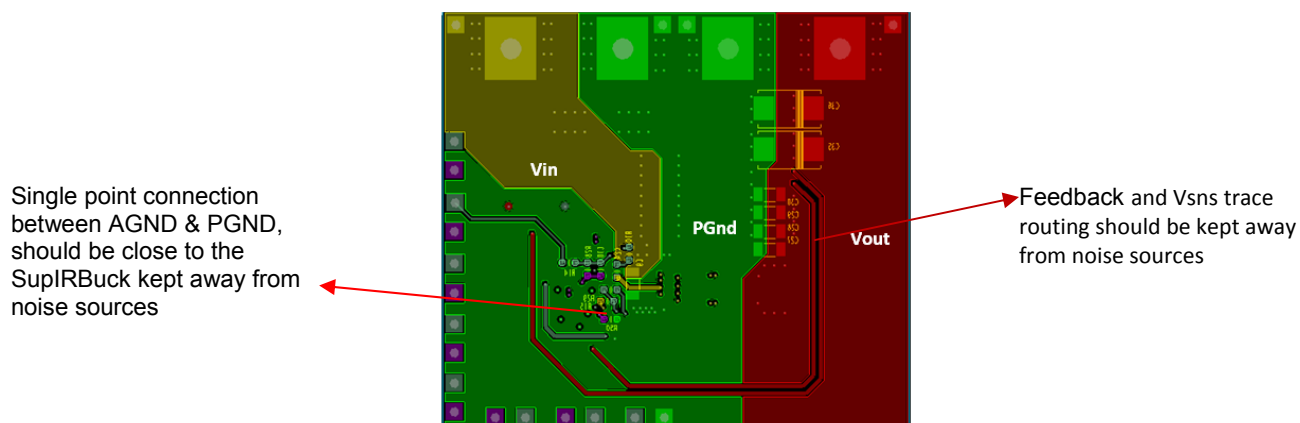
Figure 47b: IRDC3894 Demo board Layout Considerations – Bottom Layer
