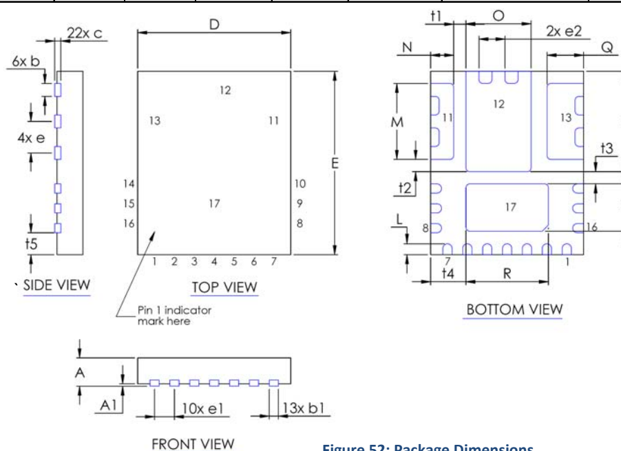
Figure 52: Package Dimensions
