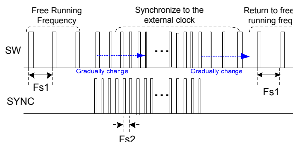
Figure 9b: Timing Diagram for Synchronization to the external clock ( F_{s1} > F_{s2} or F_{s1} < F_{s2} )
