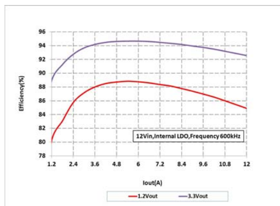
Figure 2: IR3894 Efficiency
