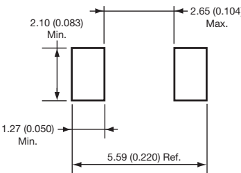
DO-214AA (SMB)
