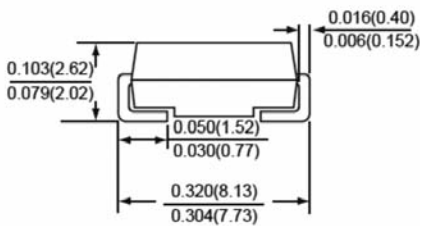
SMC/DO-214AB
