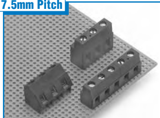
7.5mm Pitch
