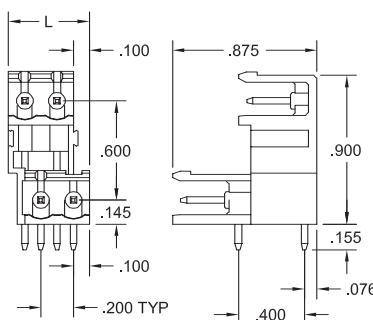
ELFD—Horizontal
