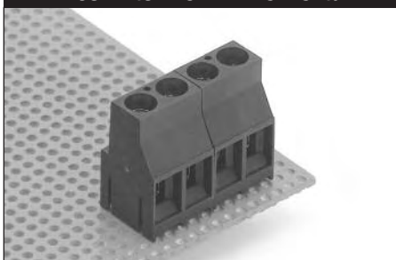
.250" Pitch ESPM—Horizontal
