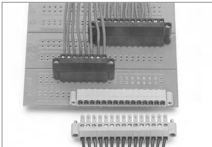
ELVH Horizontal—Eared
