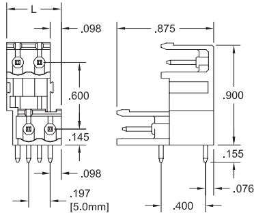
ELFD—Horizontal
