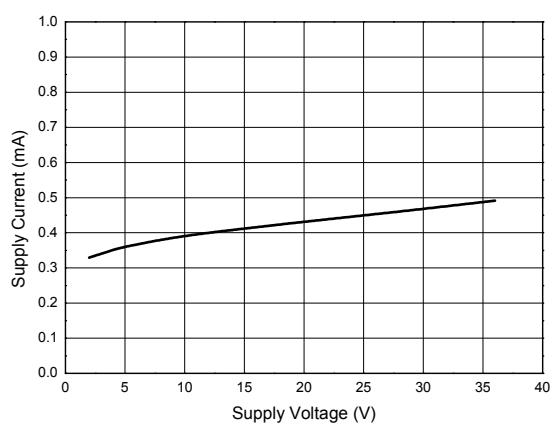
Figure 6. Supply Current
