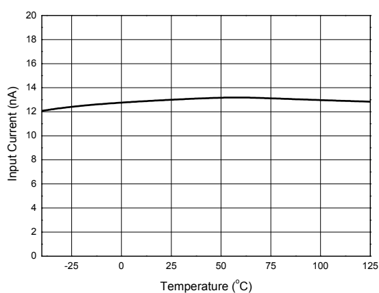
Figure 5. Input Current
