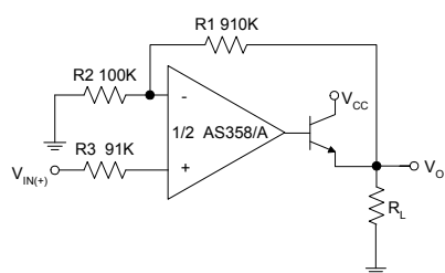
Figure 16. Power Amplifier
